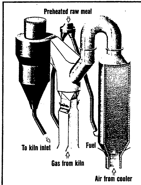
SLC-S calciner.
